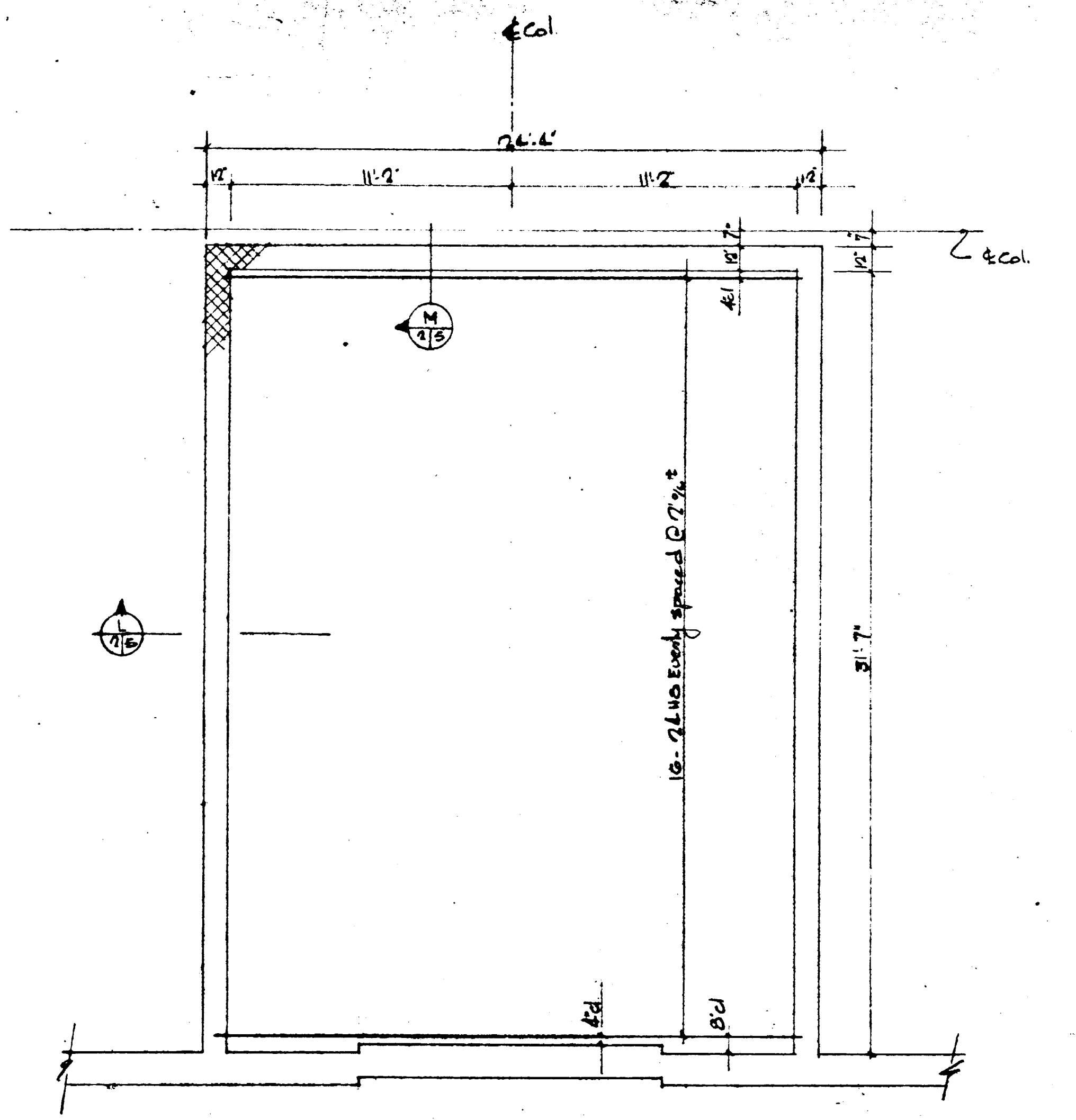
FLOOR OVER OFFICE FRAMING PLAN 1/2"x11'-0"
