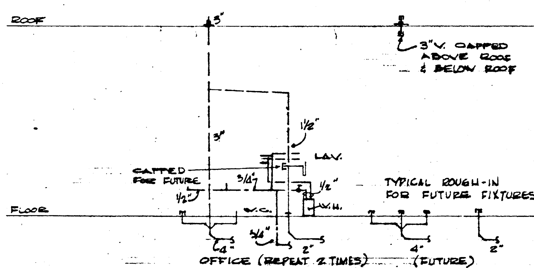
SANITARY DRAINAGE DIAGRAM NO SCALE
