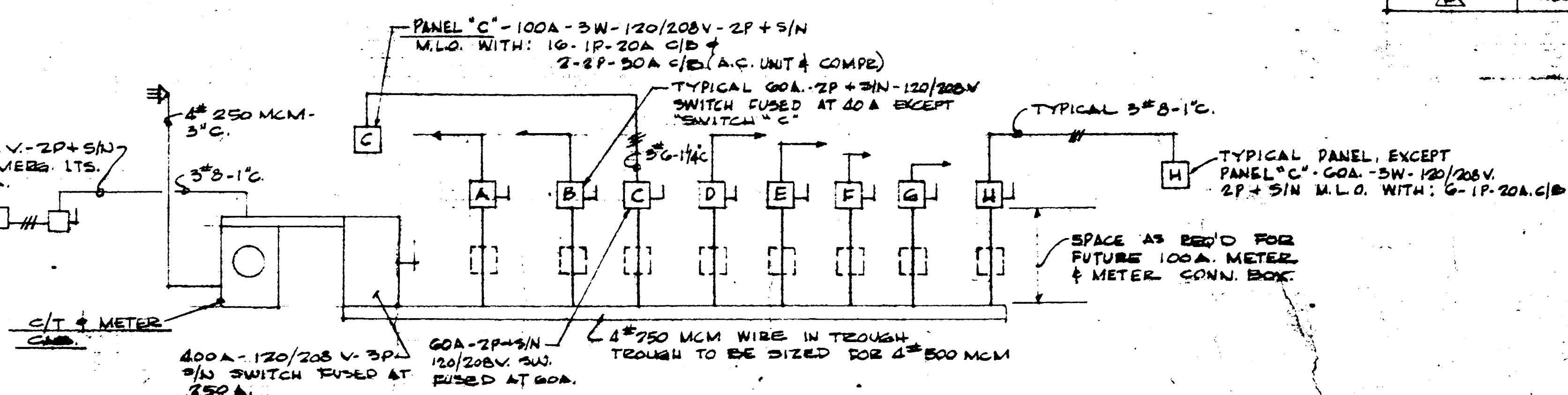
ELECTRICAL RISER DIAGRAM NO SCALE
